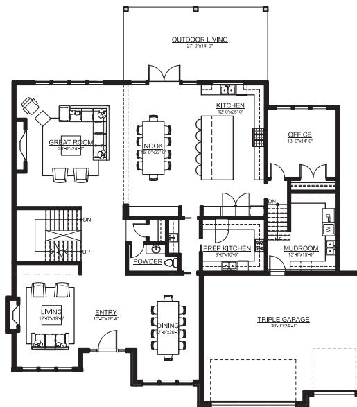
MAIN FLOOR 2810 SF
